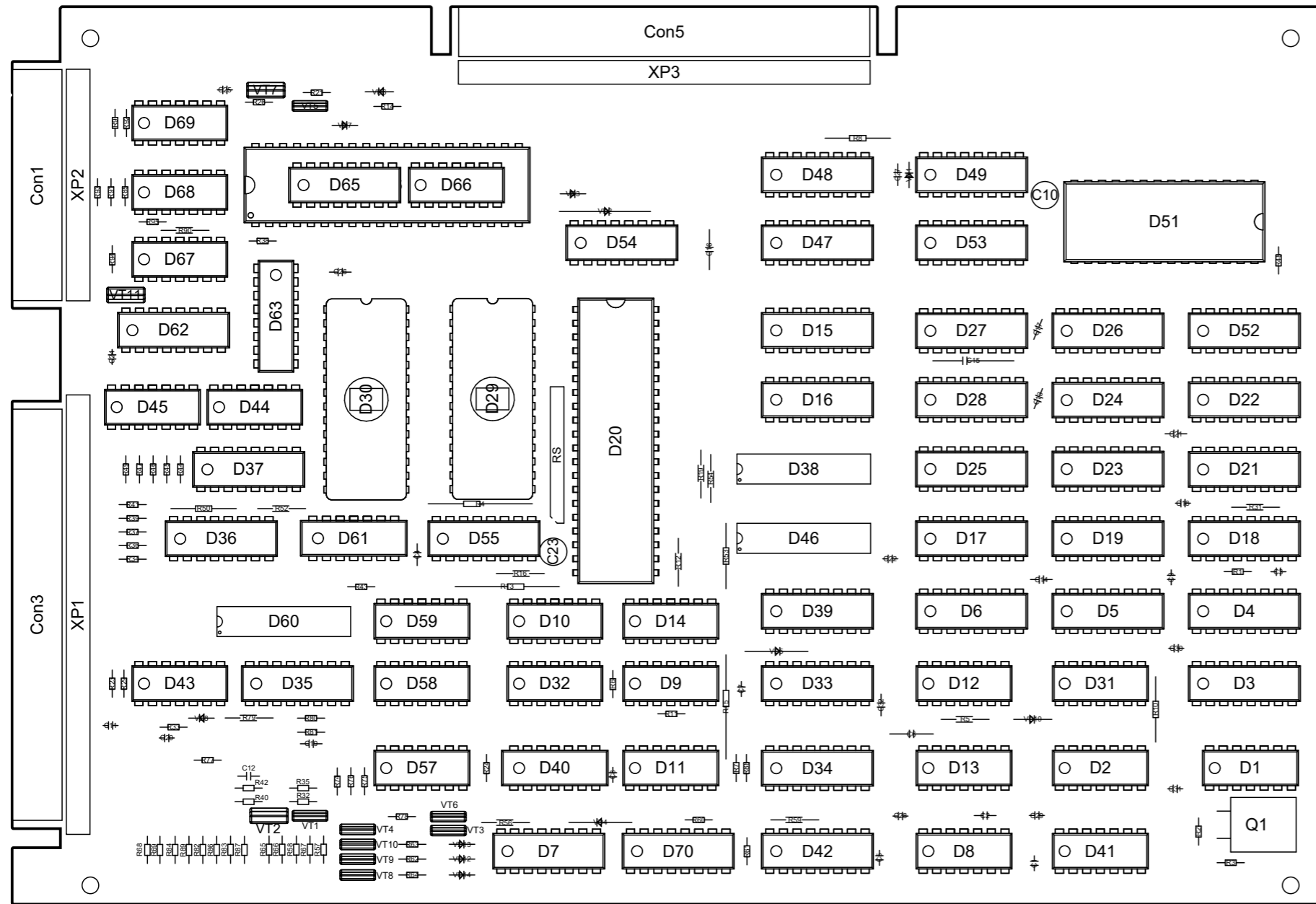
View from Top side (Scale 1:1)
